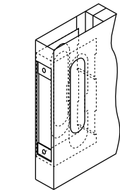
ANSI / SDI A115.1 "MB" (MORTISE)
